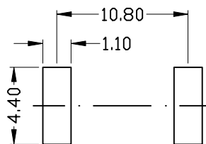
(MOUNTING DETAIL)
