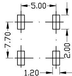
(MOUNTING DETAIL)
