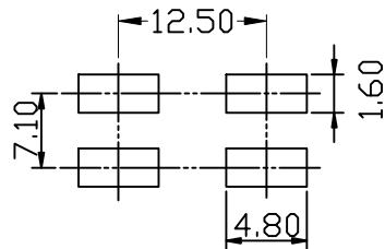
(MOUNTING DETAIL)
