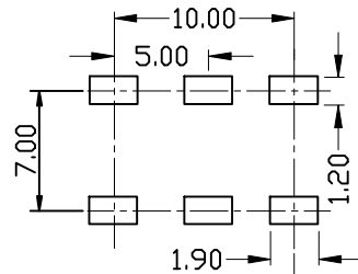
(MOUNTING DETAIL)
