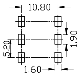
(MOUNTING DETAIL)
